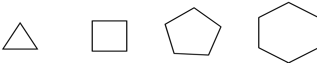
Cyclopropane
