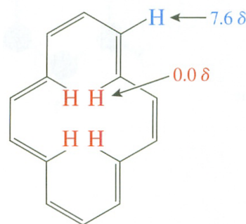
[14]Annulene
