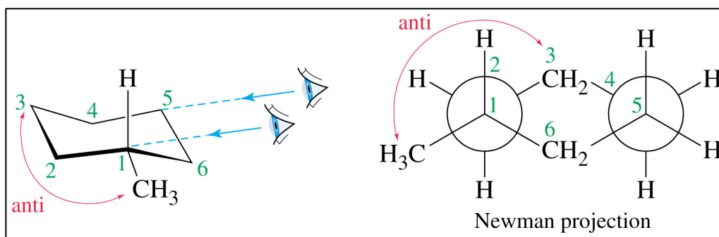
Equatorial methyl cyclohexane
