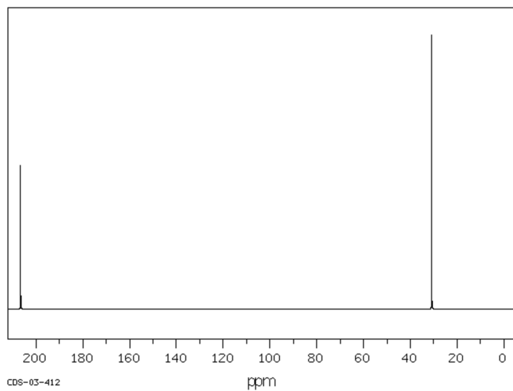
C-13 NMR spectrum of acetone
