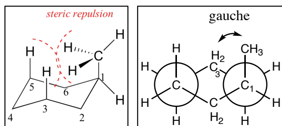
Axial methyl cyclohexane
