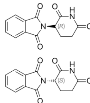
Thalidomide
