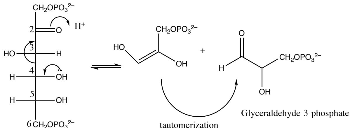
Fructose-1,6-diphosphate
