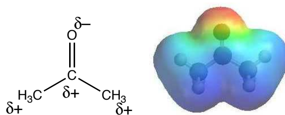
Two representations of acetone showing the distribution of charge
