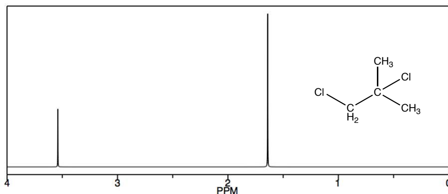
1 H NMR Spectrum of 1,2-dichloro-2-methylpropane
