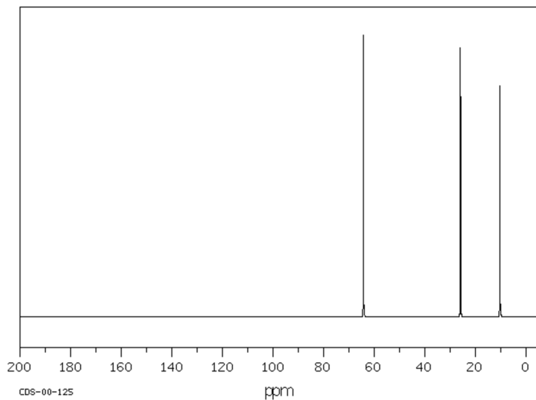
C-13 Spectrum of 1-propanol
